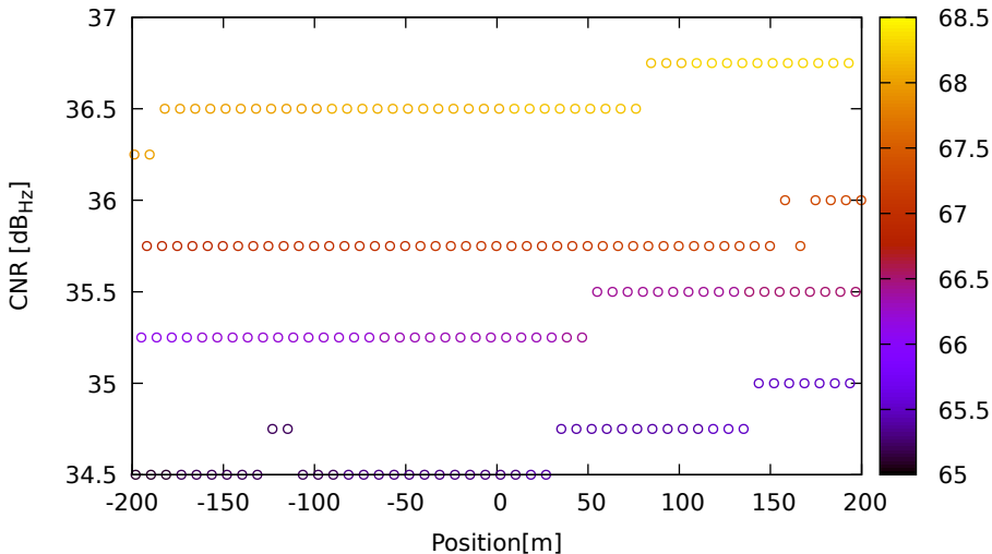
CNR vs position for G04 (L5) on Xiaomi11T - DOY 263 jam. 2
