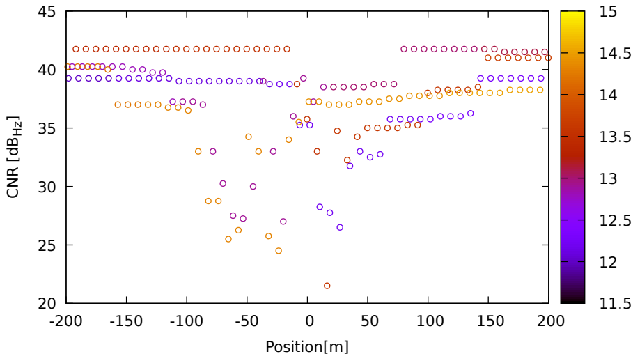
CNR vs position for G06 (L1) on Xiaomi11T - DOY 263 jam. 2
