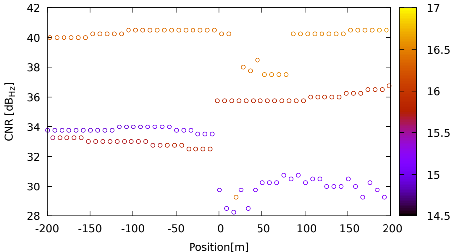
CNR vs position for G06 (L1) on Xiaomi11T - DOY 263 jam. 3
