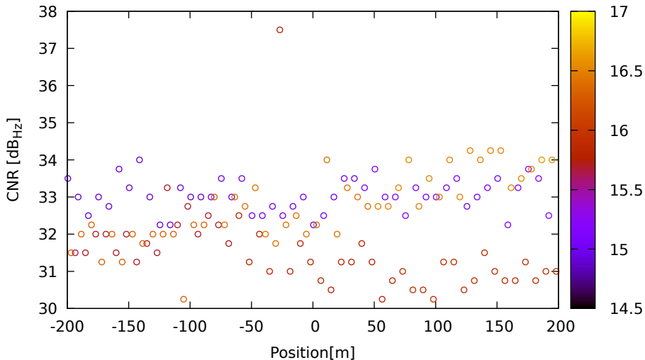
CNR vs position for G06 (L5) on Xiaomi11T - DOY 263 jam. 3
