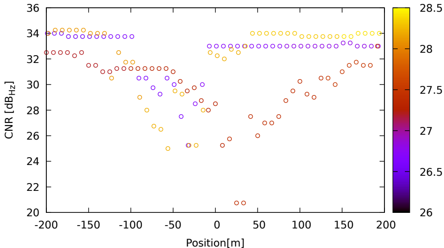
CNR vs position for G09 (L1) on Xiaomi11T - DOY 263 jam. 1
