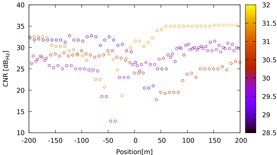
CNR vs position for G09 (L1) on Xiaomi11T - DOY 263 jam. 2
