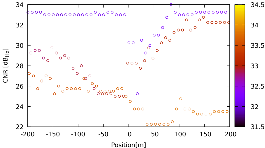
CNR vs position for G09 (L1) on Xiaomi11T - DOY 263 jam. 3
