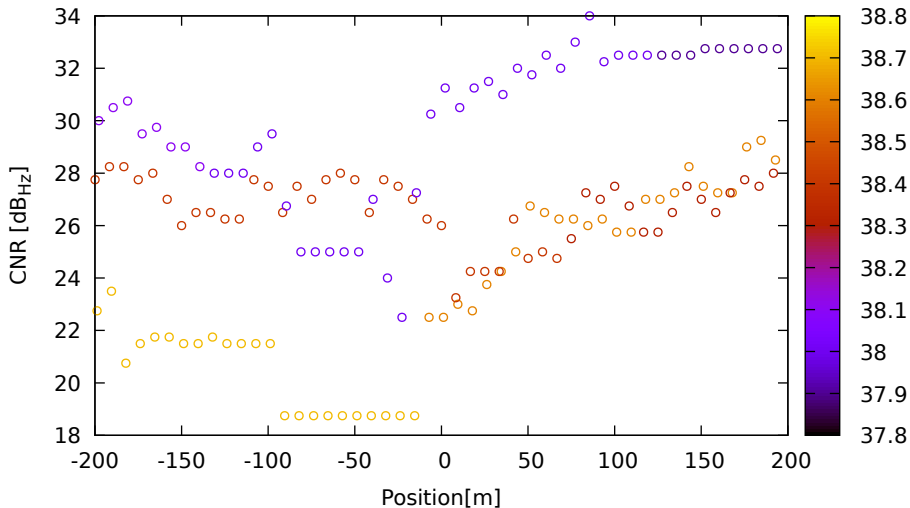
CNR vs position for G17 (L1) on Xiaomi11T - DOY 263 jam. 1
