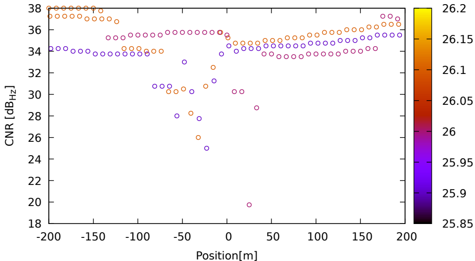
CNR vs position for G31 (L1) on Xiaomi11T - DOY 263 jam. 1
