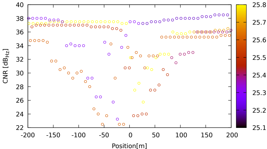
CNR vs position for G31 (L1) on Xiaomi11T - DOY 263 jam. 2
