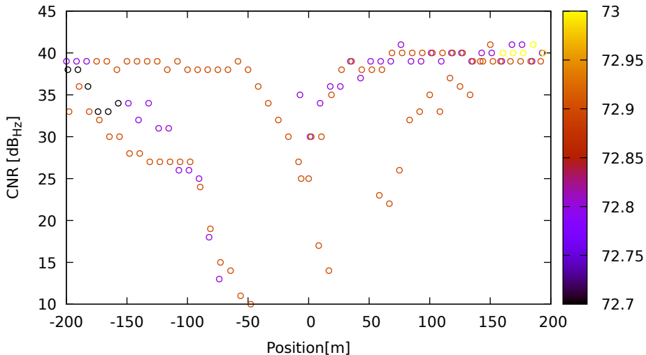
CNR vs position for R02 (G1) on Xiaomi11T - DOY 263 jam. 1
