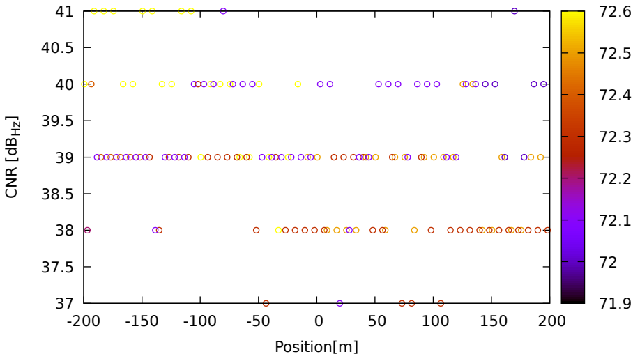
CNR vs position for R02 (G1) on Xiaomi11T - DOY 263 jam. 3
