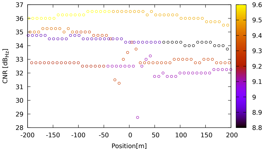
CNR vs position for R10 (G1) on Xiaomi11T - DOY 263 jam. 2
