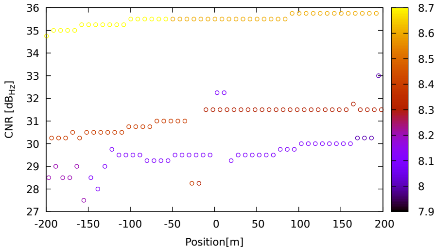
CNR vs position for R10 (G1) on Xiaomi11T - DOY 263 jam. 3
