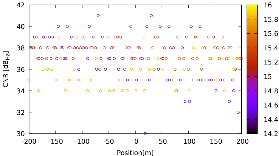
CNR vs position for R11 (G1) on Xiaomi11T - DOY 263 jam. 2
