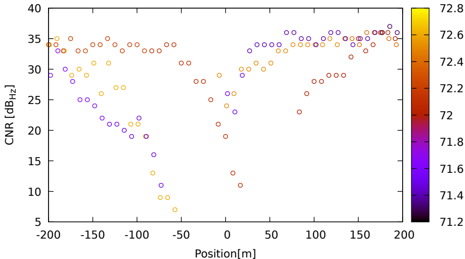
CNR vs position for R17 (G1) on Xiaomi11T - DOY 263 jam. 1
