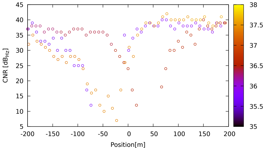
CNR vs position for R18 (G1) on Xiaomi11T - DOY 263 jam. 1
