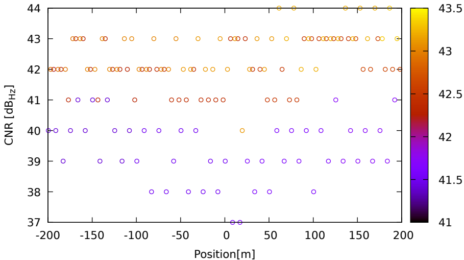
CNR vs position for R18 (G1) on Xiaomi11T - DOY 263 jam. 3
