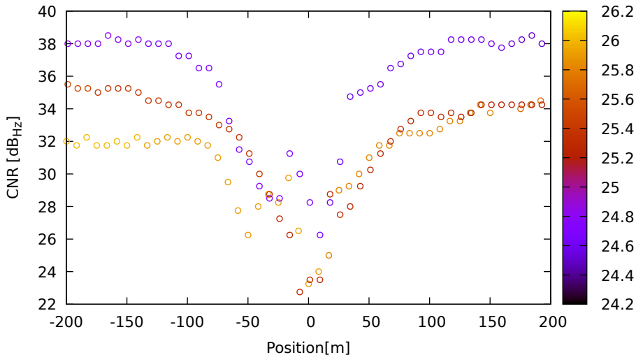
CNR vs position for C21 (B1) on XiaomiMi8 - DOY 263 jam. 1
