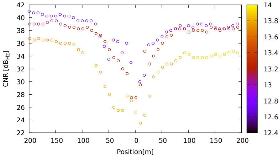
CNR vs position for C26 (B1) on XiaomiMi8 - DOY 263 jam. 1
