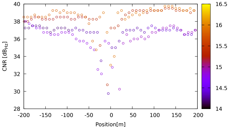
CNR vs position for C26 (B1) on XiaomiMi8 - DOY 263 jam. 2
