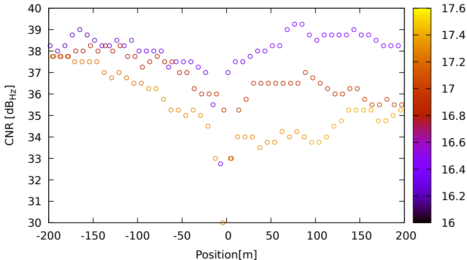
CNR vs position for C26 (B1) on XiaomiMi8 - DOY 263 jam. 3
