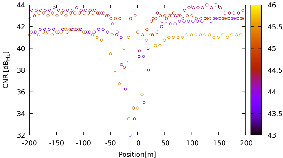
CNR vs position for C33 (B1) on XiaomiMi8 - DOY 263 jam. 2
