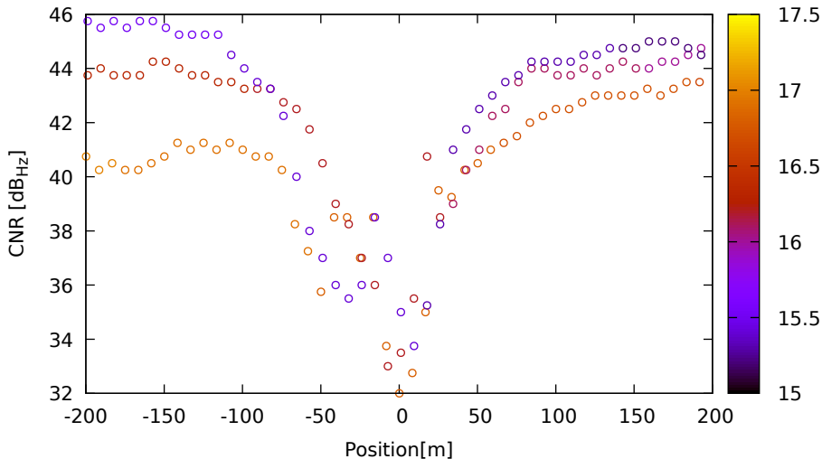
CNR vs position for C34 (B1) on XiaomiMi8 - DOY 263 jam. 1
