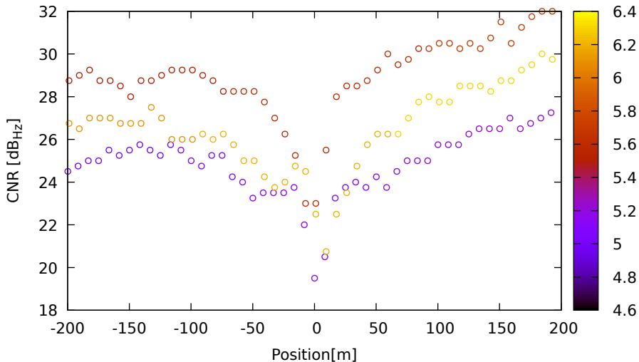
CNR vs position for E09 (E1) on XiaomiMi8 - DOY 263 jam. 1
