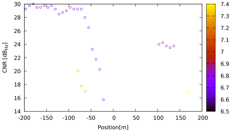
CNR vs position for E09 (E1) on XiaomiMi8 - DOY 263 jam. 2
