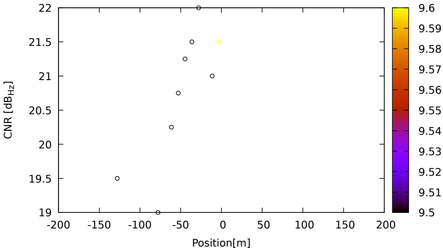
CNR vs position for E09 (E1) on XiaomiMi8 - DOY 263 jam. 3
