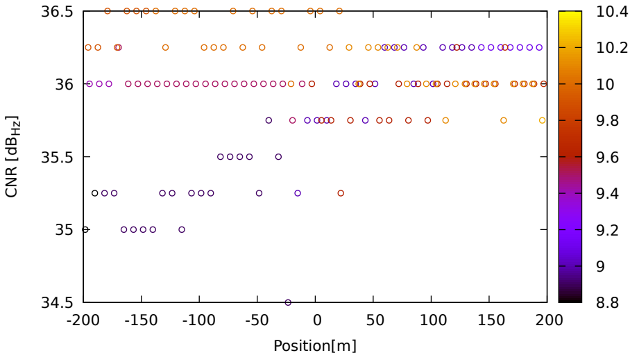
CNR vs position for E09 (E5a) on XiaomiMi8 - DOY 263 jam. 3
