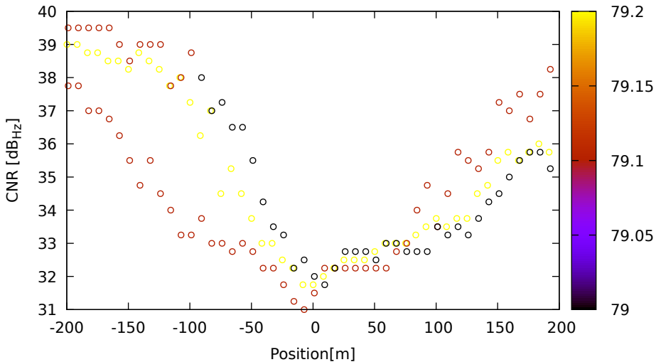
CNR vs position for E10 (E5a) on XiaomiMi8 - DOY 263 jam. 1
