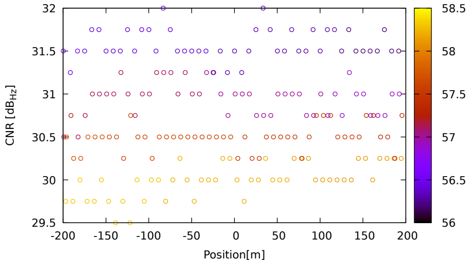
CNR vs position for E19 (E5a) on XiaomiMi8 - DOY 263 jam. 2
