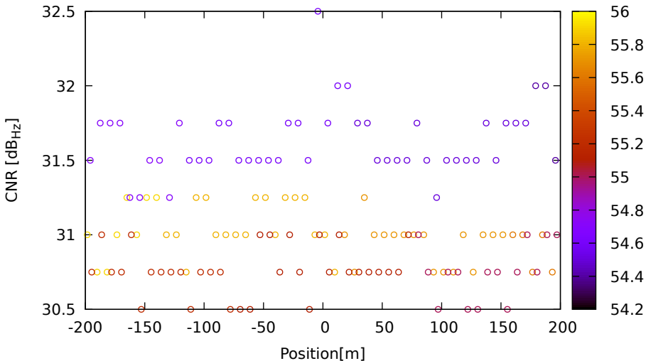
CNR vs position for E19 (E5a) on XiaomiMi8 - DOY 263 jam. 3
