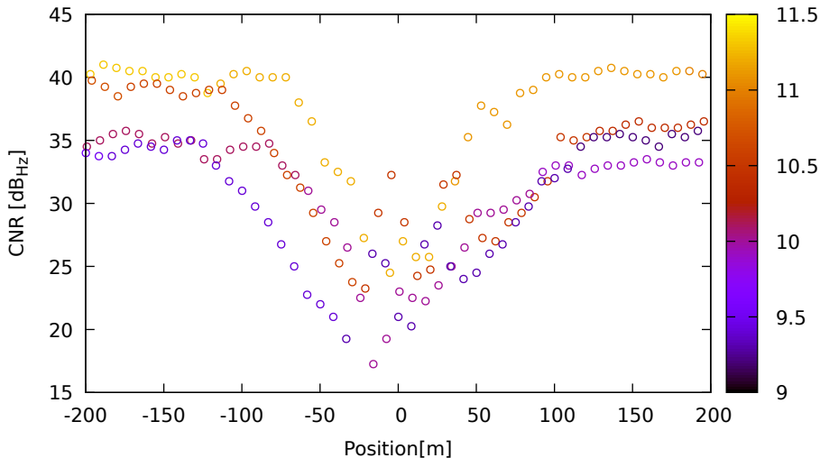
CNR vs position for E33 (E1) on XiaomiMi8 - DOY 263 jam. 2
