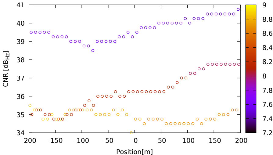
CNR vs position for E33 (E5a) on XiaomiMi8 - DOY 263 jam. 3
