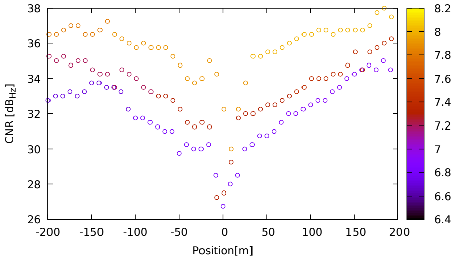
CNR vs position for E36 (E1) on XiaomiMi8 - DOY 263 jam. 1
