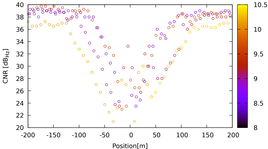
CNR vs position for E36 (E1) on XiaomiMi8 - DOY 263 jam. 2
