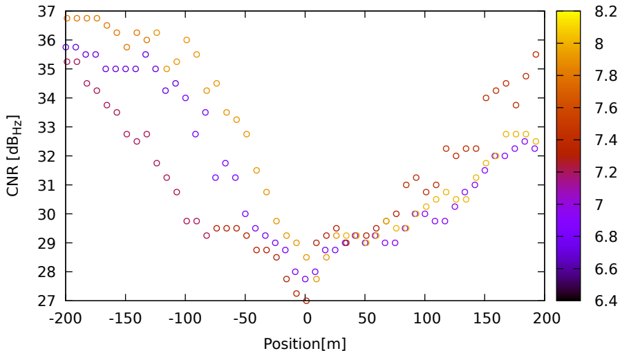
CNR vs position for E36 (E5a) on XiaomiMi8 - DOY 263 jam. 1
