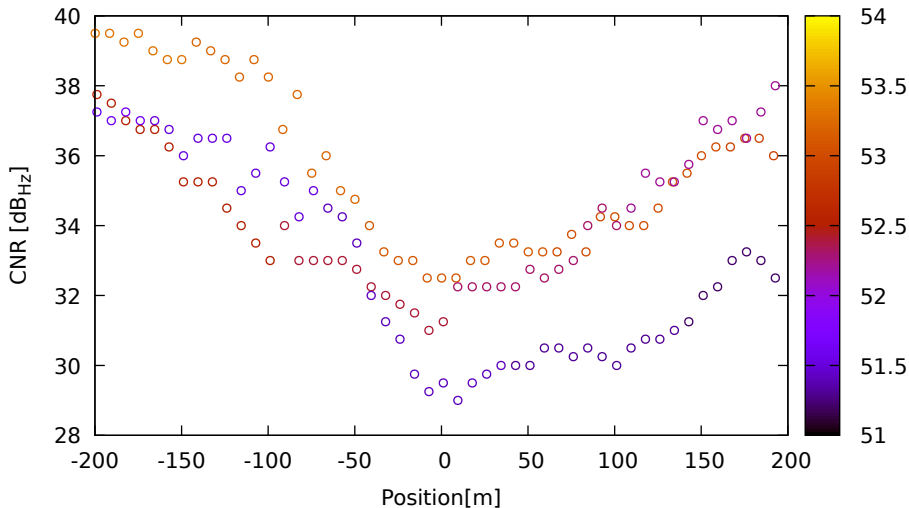
CNR vs position for G01 (L5) on XiaomiMi8 - DOY 263 jam. 1
