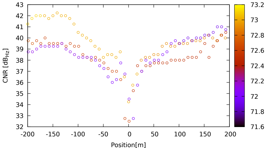
CNR vs position for G03 (L1) on XiaomiMi8 - DOY 263 jam. 1
