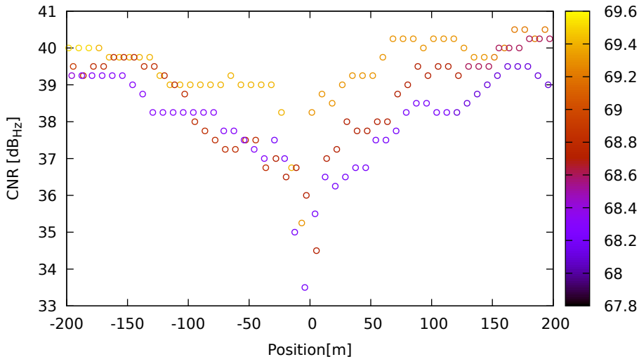
CNR vs position for G03 (L1) on XiaomiMi8 - DOY 263 jam. 3
