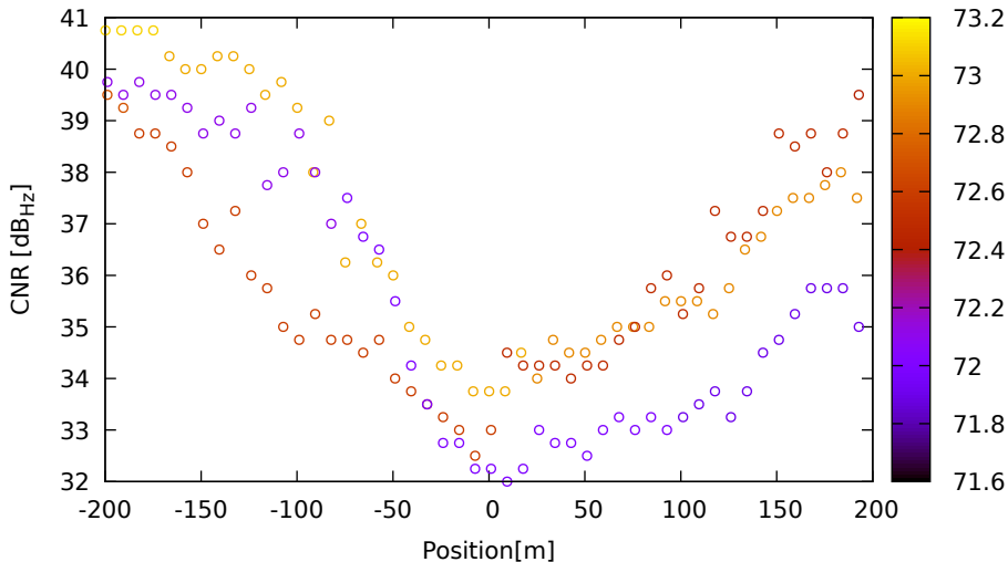
CNR vs position for G03 (L5) on XiaomiMi8 - DOY 263 jam. 1
