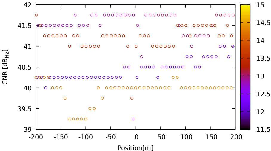
CNR vs position for G06 (L5) on XiaomiMi8 - DOY 263 jam. 2
