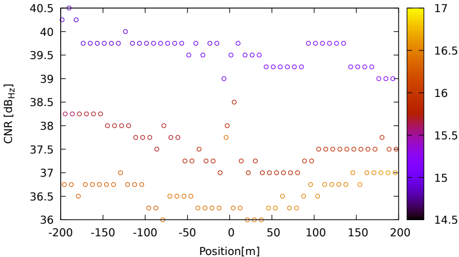
CNR vs position for G06 (L5) on XiaomiMi8 - DOY 263 jam. 3
