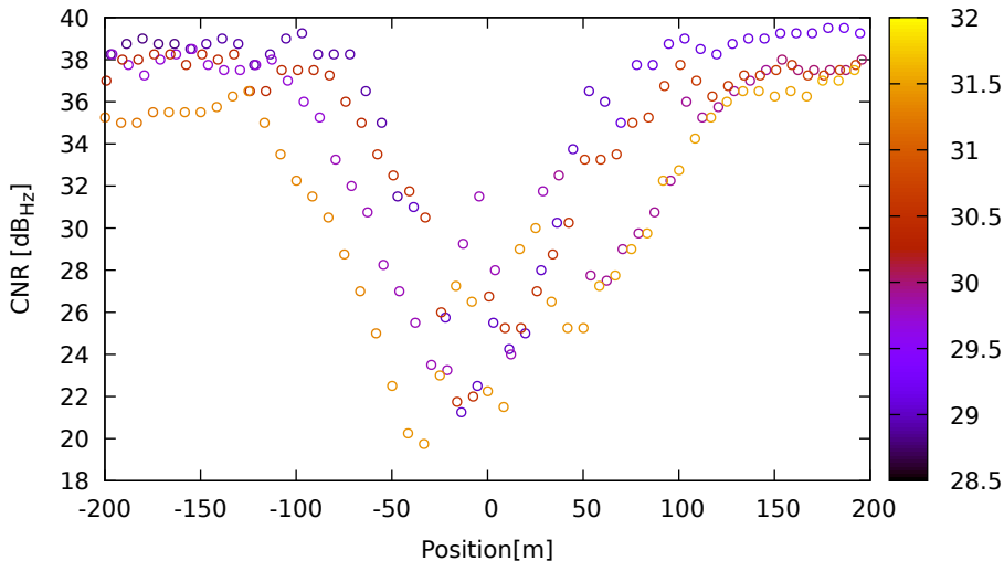
CNR vs position for G09 (L1) on XiaomiMi8 - DOY 263 jam. 2
