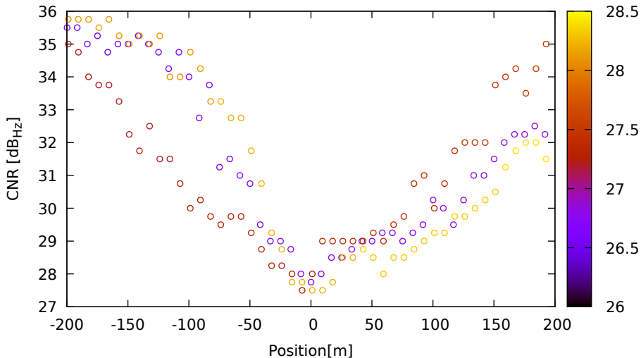
CNR vs position for G09 (L5) on XiaomiMi8 - DOY 263 jam. 1
