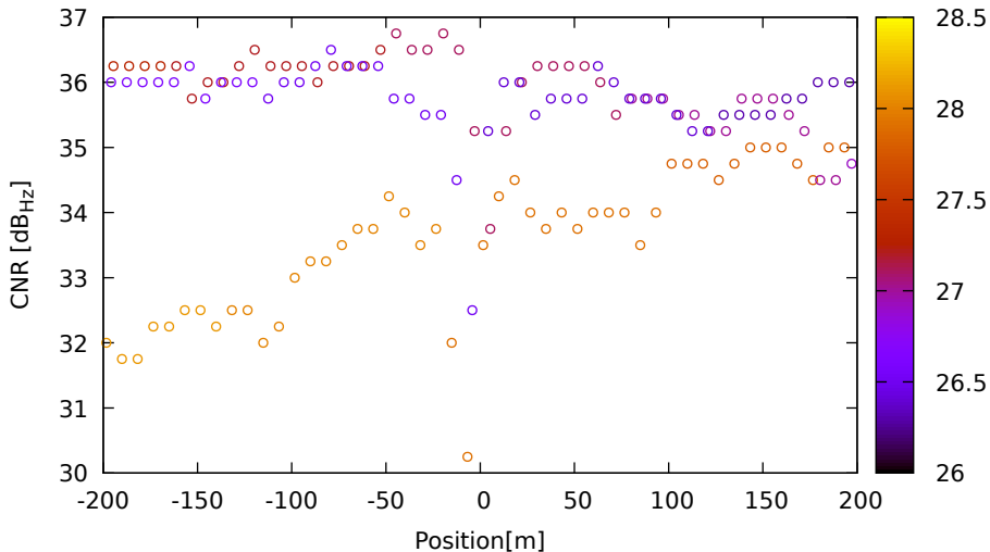
CNR vs position for R01 (G1) on XiaomiMi8 - DOY 263 jam. 3
