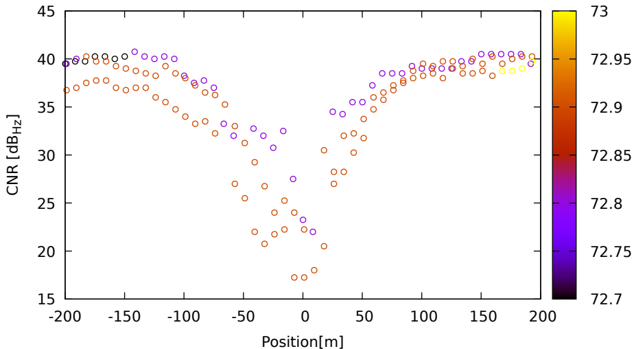
CNR vs position for R02 (G1) on XiaomiMi8 - DOY 263 jam. 1
