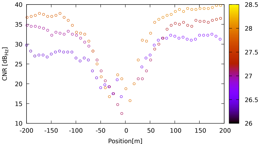
CNR vs position for R03 (G1) on XiaomiMi8 - DOY 263 jam. 1
