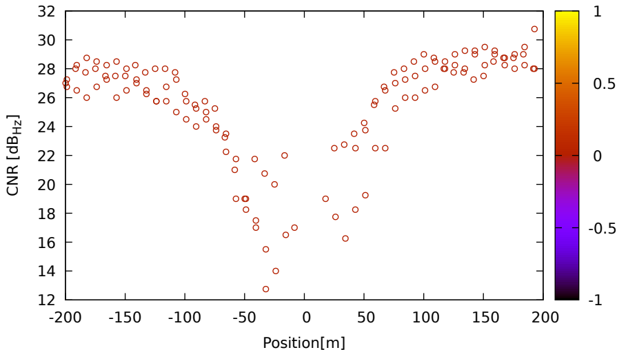
CNR vs position for R10 (G1) on XiaomiMi8 - DOY 263 jam. 1
