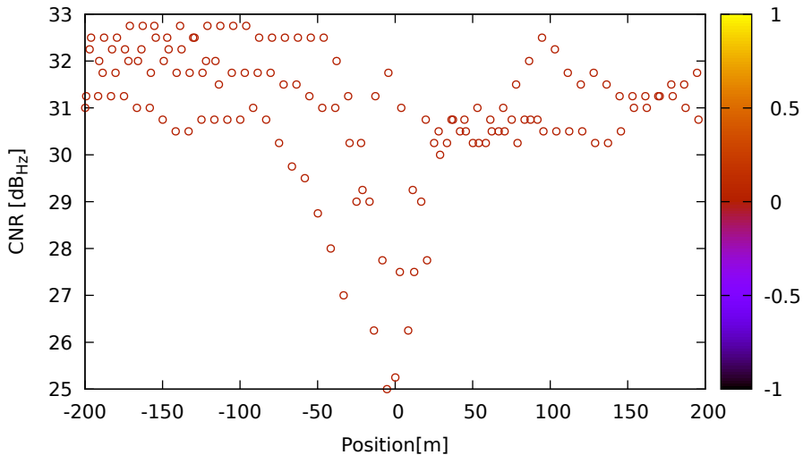
CNR vs position for R10 (G1) on XiaomiMi8 - DOY 263 jam. 2
