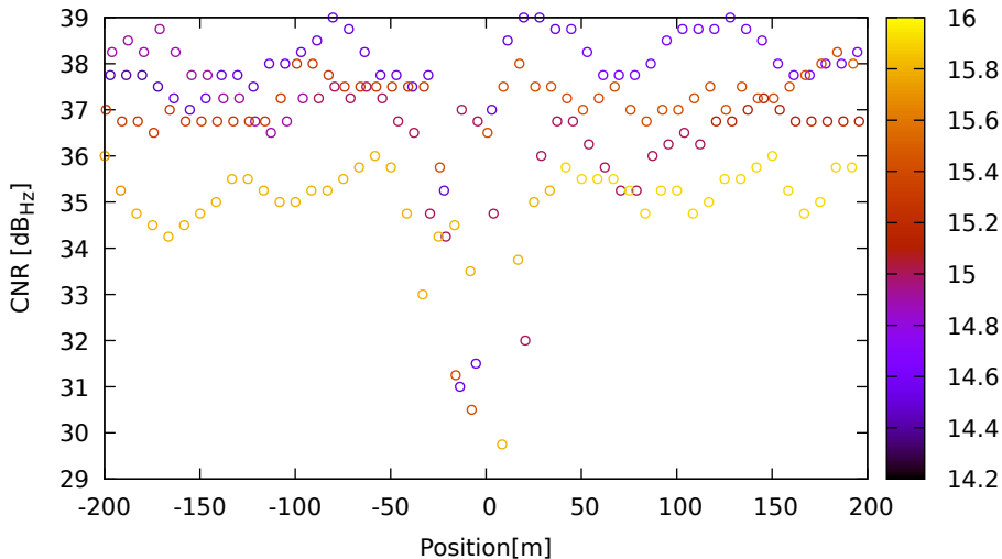
CNR vs position for R11 (G1) on XiaomiMi8 - DOY 263 jam. 2
